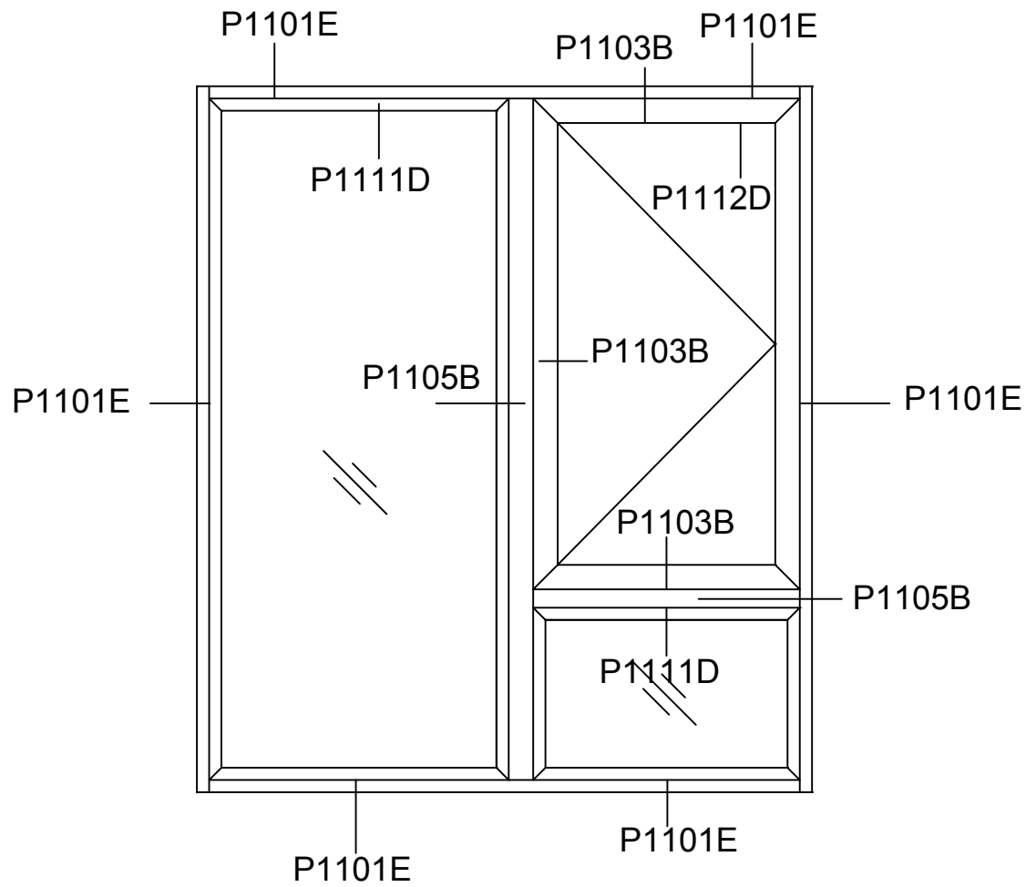
50 Casement Window Section
